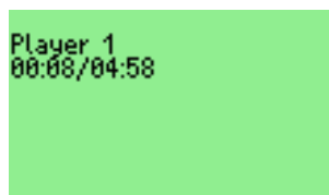
Figure 12.45.: Chess Clock
