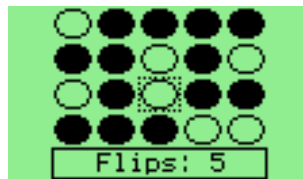
Figure 12.6.: Flipit
