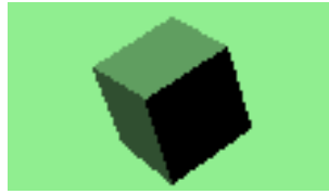
Figure 12.27.: Cube
