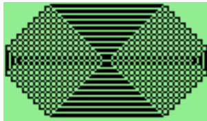
Figure 12.31.: Mosaique
