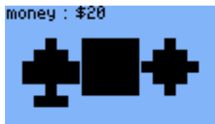
Figure 12.8.: Jackpot
