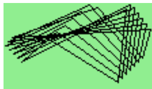
Figure 12.28.: Demystify
