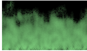
Figure 12.29.: Fire
