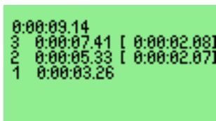
Figure 12.49.: Stopwatch
