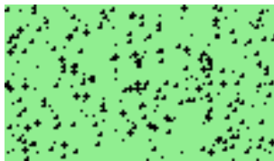
Figure 12.36.: Starfield
