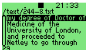
Figure 12.41.: A bookmark
