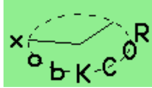
Figure 12.26.: Bounce
