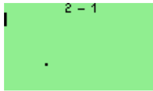
Figure 12.13.: Pong
