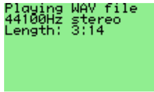
Figure 11.44.: Wavplay
